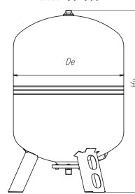
WAV 50-500
